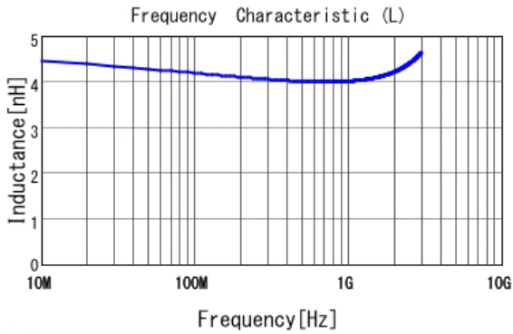
■ LQP03TN4N0B02 L
