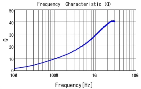
■ LQP03TN4N0B02 Q
