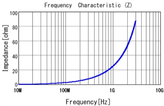
■ LQP03TN4N0B02 |Z|
