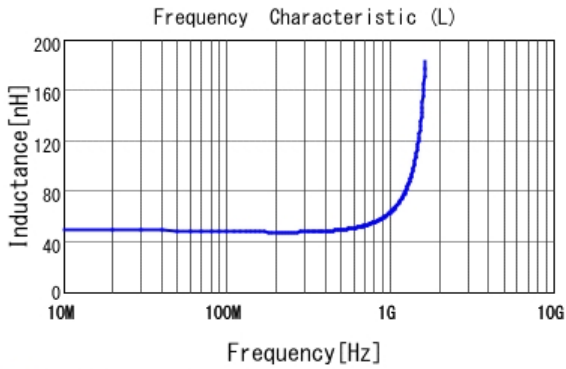
■ LQP03TN47NH02 L
