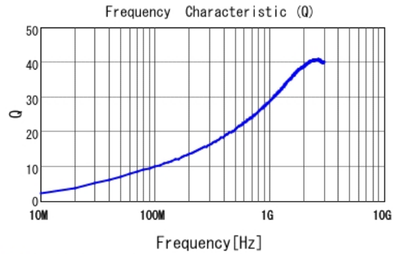
■ LQP03TN3N7B02 Q
