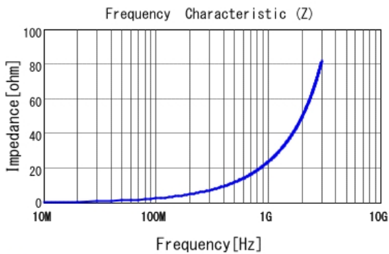
■ LQP03TN3N7B02 |Z|
