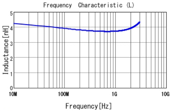
■ LQP03TN3N7B02 L
