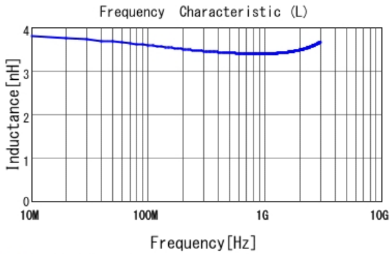
■ LQP03TN3N4B02 L
