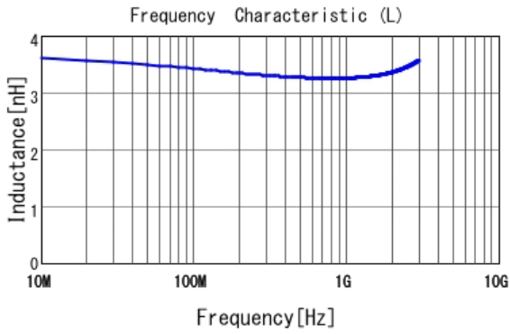
■ LQP03TN3N3C02 L
