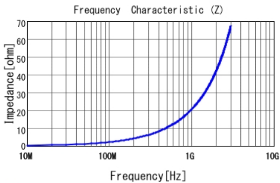
■ LQP03TN3N3C02 |Z|
