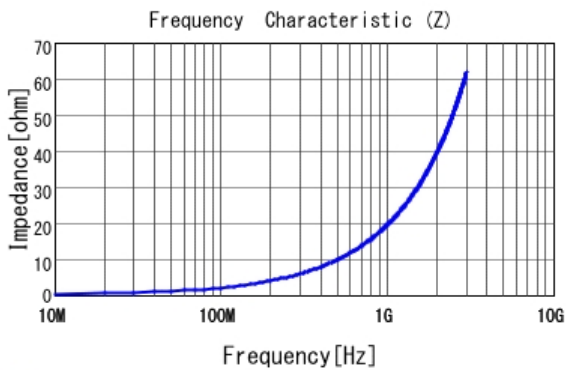
■ LQP03TN3N1B02 |Z|
