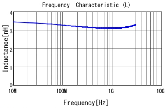
■ LQP03TN3N1B02 L
