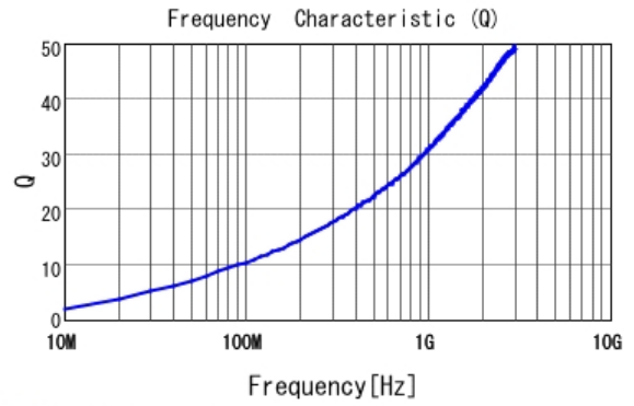
■ LQP03TN3N1B02 Q
