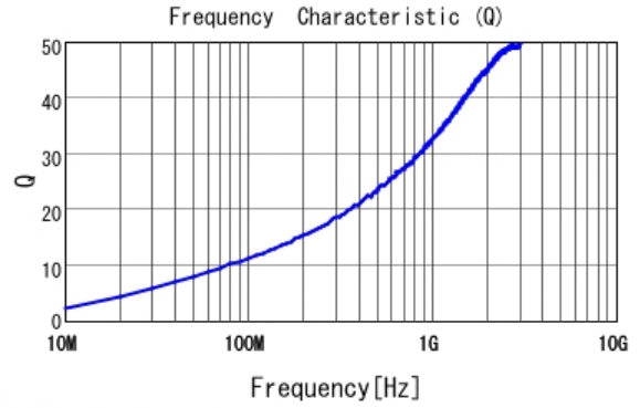
■ LQP03TN3N0C02 Q
