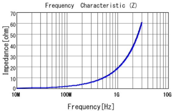
■ LQP03TN3N0C02 |Z|
