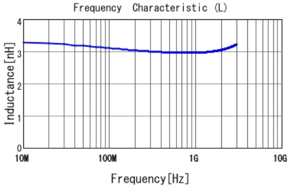
■ LQP03TN3N0C02 L
