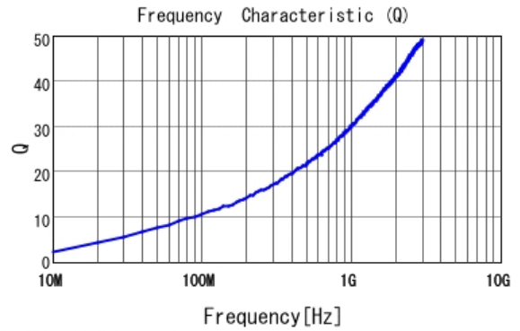
■ LQP03TN2N8B02 Q
