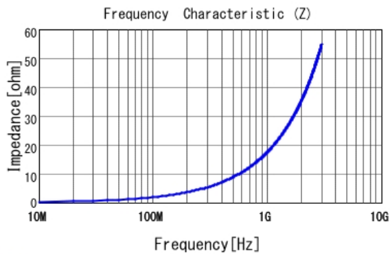
■ LQP03TN2N8B02 |Z|
