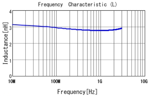
■ LQP03TN2N8B02 L
