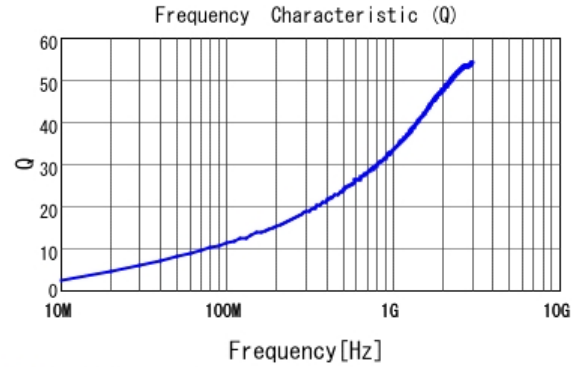
■ LQP03TN2N1B02 Q
