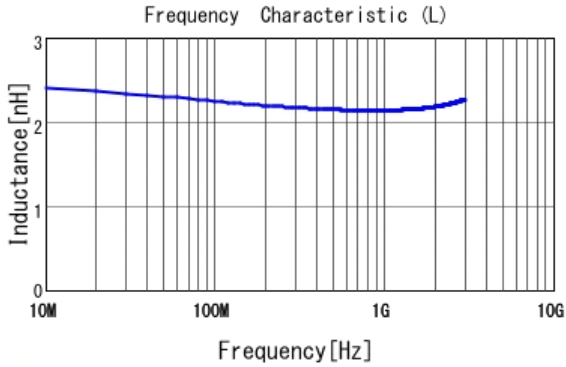
■ LQP03TN2N1B02 L
