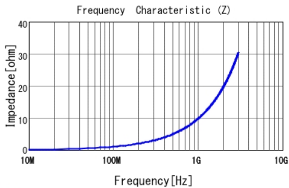
■ LQP03TN1N5C02 |Z|
