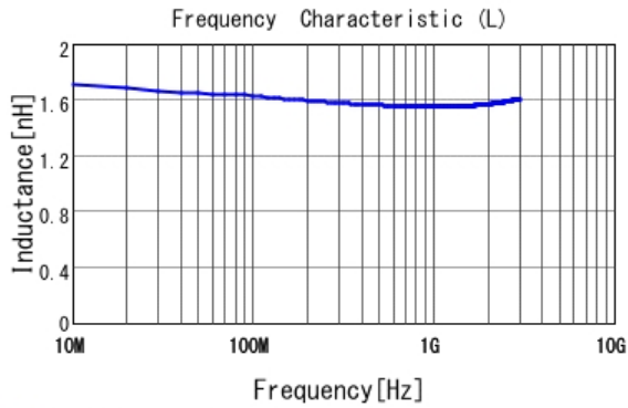
■ LQP03TN1N5C02 L
