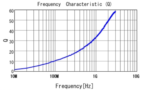
■ LQP03TN1N5C02 Q
