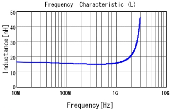
■ LQP03TN15NJ02 L
