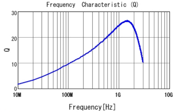
■ LQP03TN15NJ02 Q
