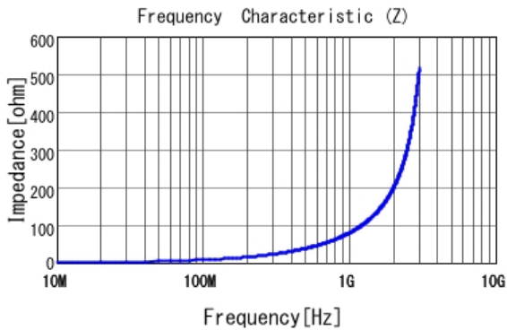
■ LQP03TN12NJ02 |Z|
