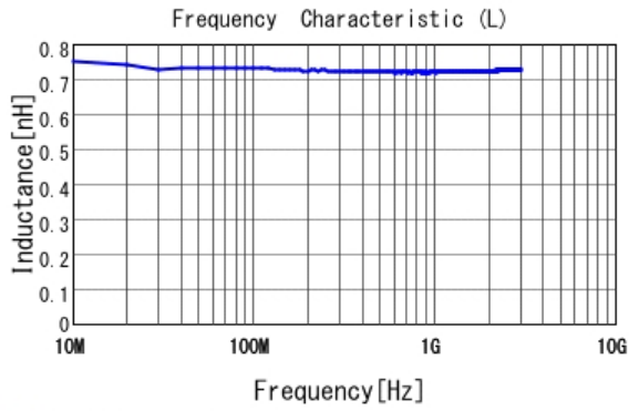
■ LQP03TN0N7B02 L
