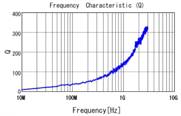
■ LQP03TN0N7B02 Q
