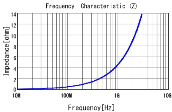
■ LQP03TN0N7B02 |Z|
