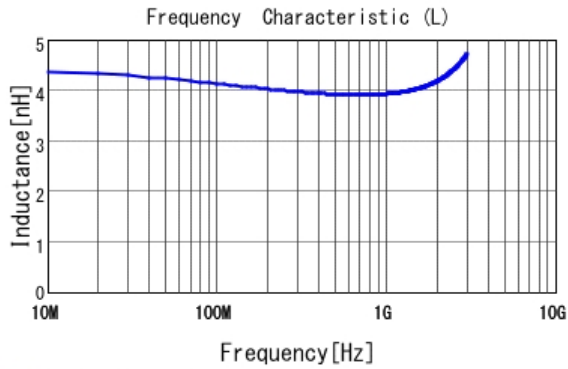
■ LQP03TG3N9B02 L
