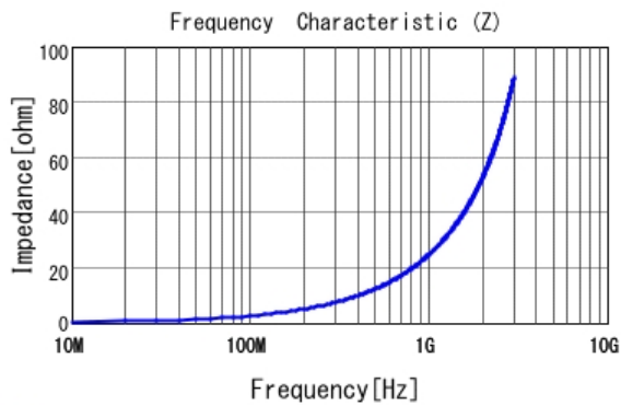
■ LQP03TG3N9B02 |Z|
