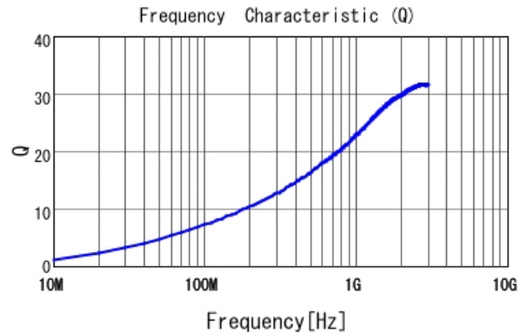
■ LQP03TG3N9B02 Q
