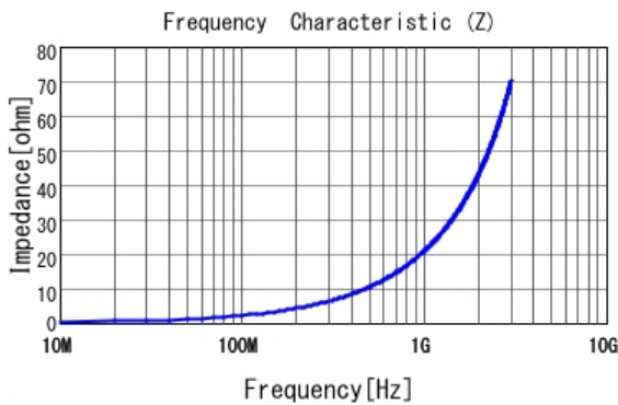
■ LQP03TG3N3B02 |Z|
