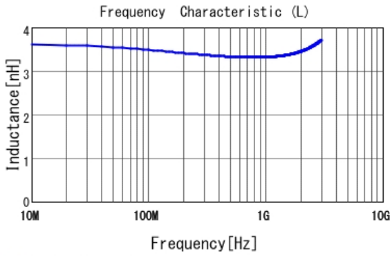
■ LQP03TG3N3B02 L
