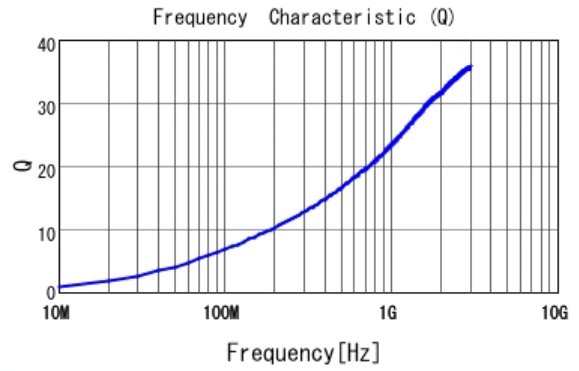
■ LQP03TG3N3B02 Q
