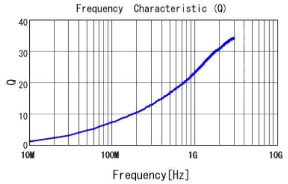
■ LQP03TG3N0B02 Q
