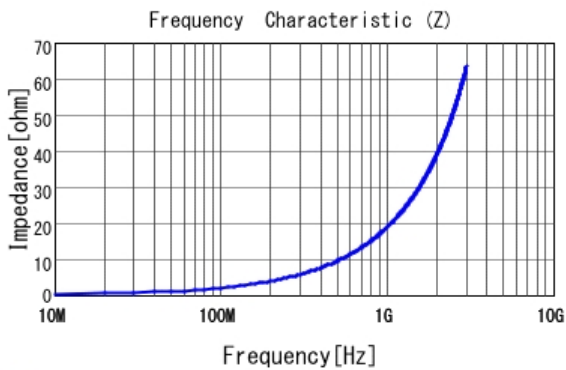
■ LQP03TG3N0B02 |Z|
