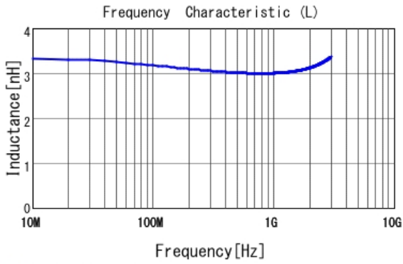
■ LQP03TG3N0B02 L
