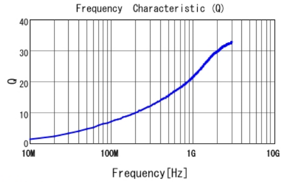
■ LQP03TG2N7B02 Q
