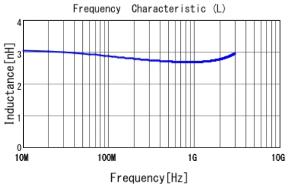
■ LQP03TG2N7B02 L
