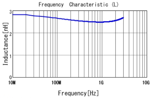
■ LQP03TG2N5C02 L
