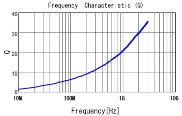
■ LQP03TG1N1B02 Q
