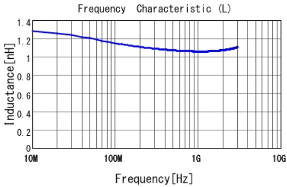
■ LQP03TG1N1B02 L
