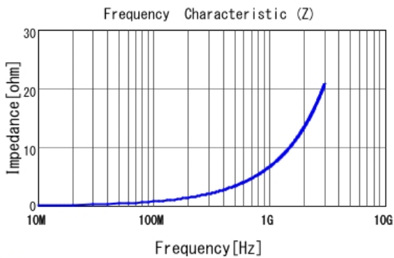
■ LQP03TG1N1B02 |Z|
