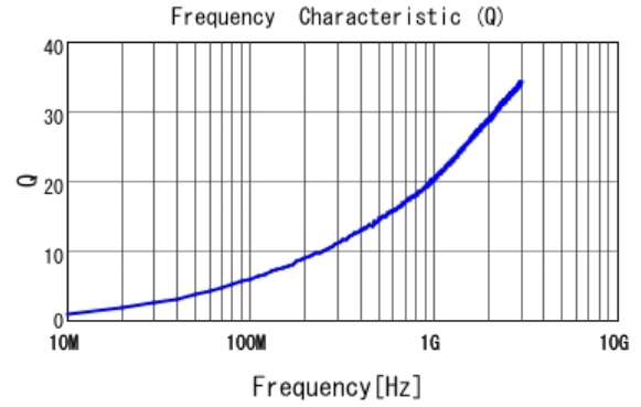
■ LQP03TG1N0B02 Q
