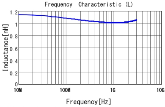
■ LQP03TG1N0B02 L
