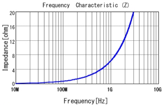
■ LQP03TG1N0B02 |Z|
