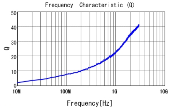
■ LQP03TG0N5B02 Q
