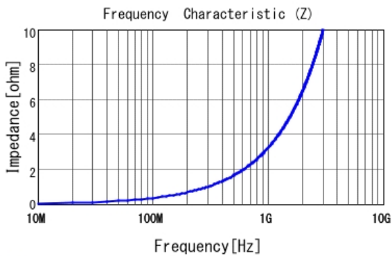
■ LQP03TG0N5B02 |Z|
