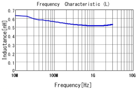
■ LQP03TG0N5B02 L
