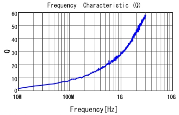
■ LQP03TG0N3B02 Q
