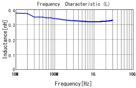
■ LQP03TG0N3B02 L
