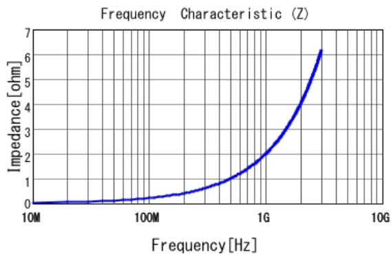
■ LQP03TG0N3B02 |Z|
