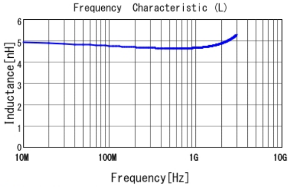
■ LQP03HQ4N7J02 L
