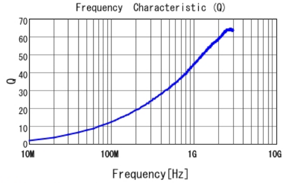
■ LQP03HQ4N7J02 Q
