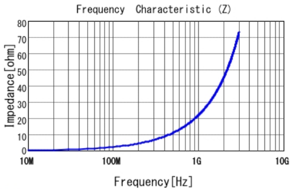
■ LQP03HQ3N5B02 |Z|
