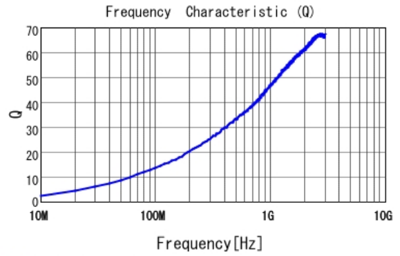
■ LQP03HQ3N5B02 Q
