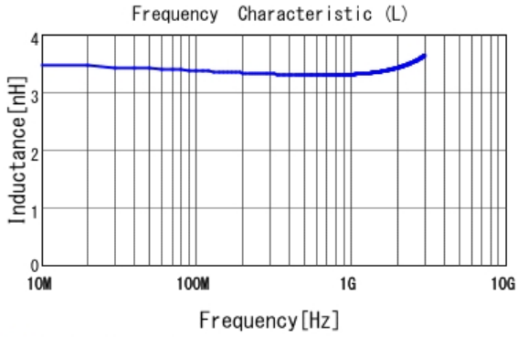
■ LQP03HQ3N3B02 L
