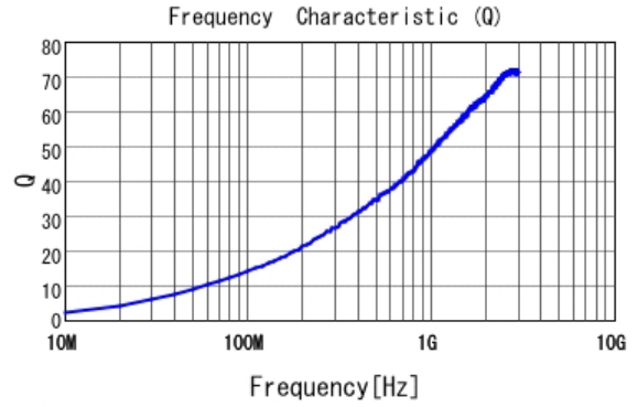
■ LQP03HQ3N3B02 Q
