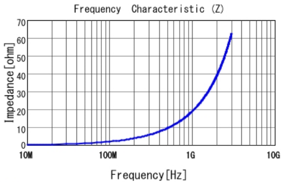
■ LQP03HQ3N0B02 |Z|
