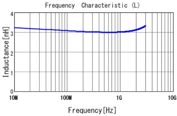
■ LQP03HQ3N0B02 L
