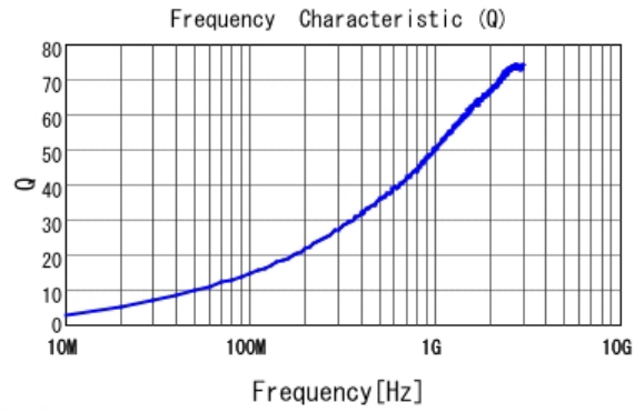
■ LQP03HQ3N0B02 Q
