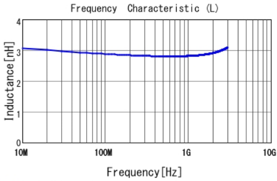
■ LQP03HQ2N8B02 L
