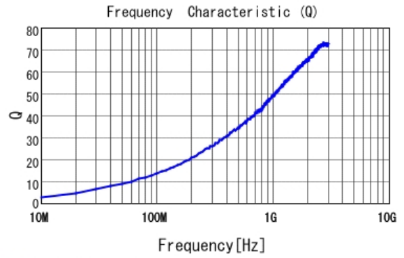
■ LQP03HQ2N8B02 Q
