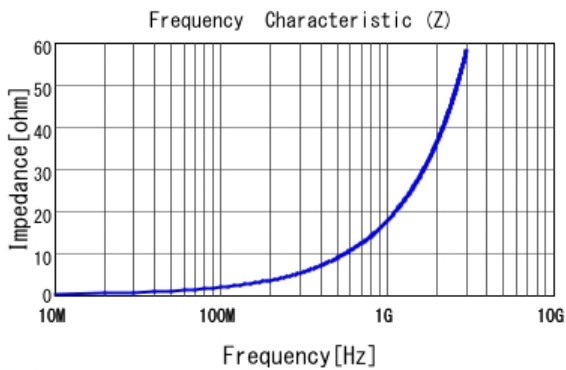
■ LQP03HQ2N8B02 |Z|
