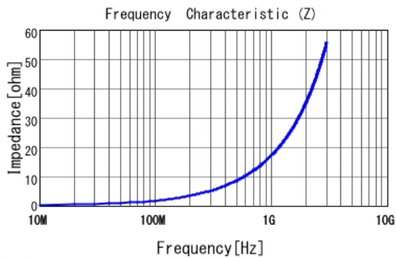
■ LQP03HQ2N7B02 |Z|
