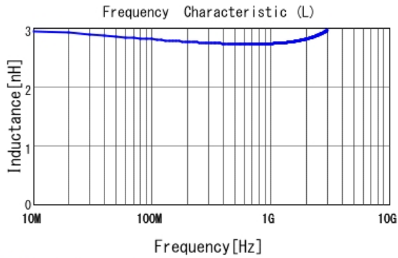
■ LQP03HQ2N7B02 L
