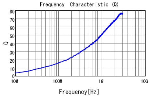
■ LQP03HQ2N7B02 Q
