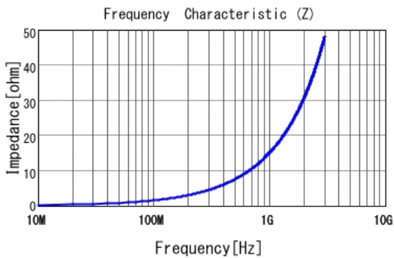
■ LQP03HQ2N4B02 |Z|
