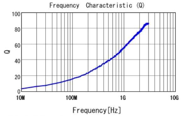
■ LQP03HQ2N4B02 Q
