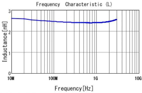
■ LQP03HQ2N4B02 L
