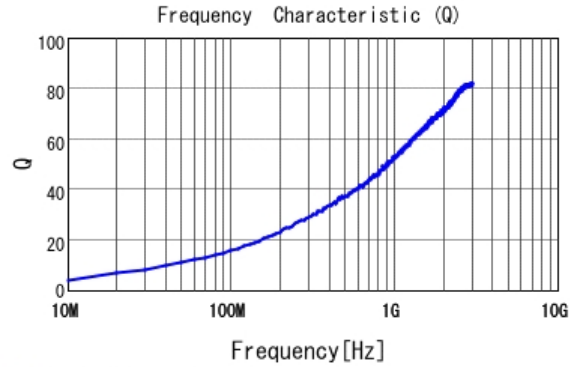
■ LQP03HQ2N3B02 Q
