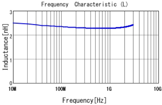
■ LQP03HQ2N3B02 L
