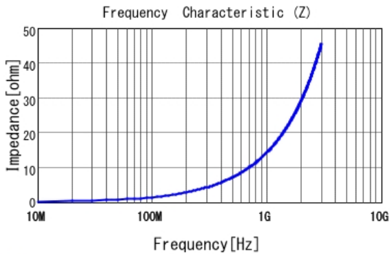
■ LQP03HQ2N3B02 |Z|
