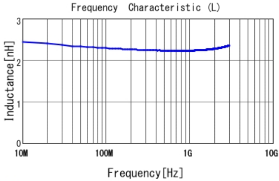
■ LQP03HQ2N2W02 L
