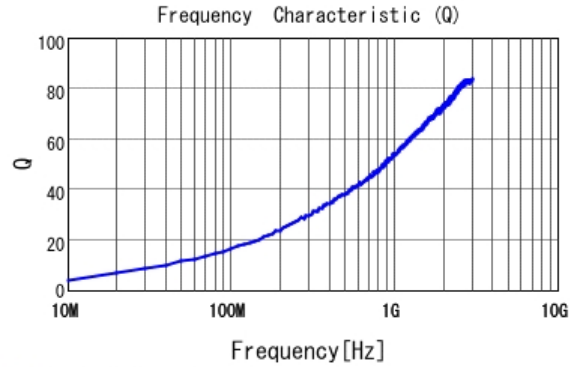
■ LQP03HQ2N2W02 Q
