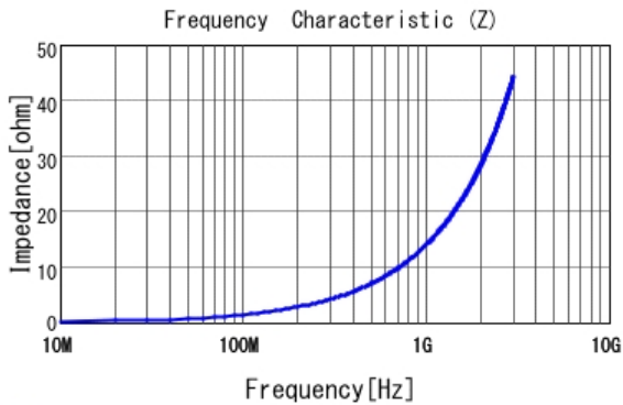
■ LQP03HQ2N2W02 |Z|
