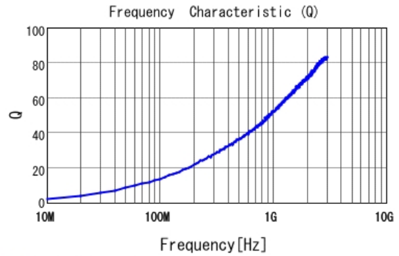
■ LQP03HQ2N0B02 Q
