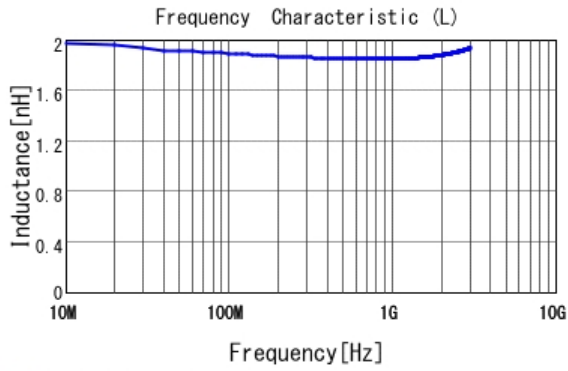
■ LQP03HQ1N8W02 L
