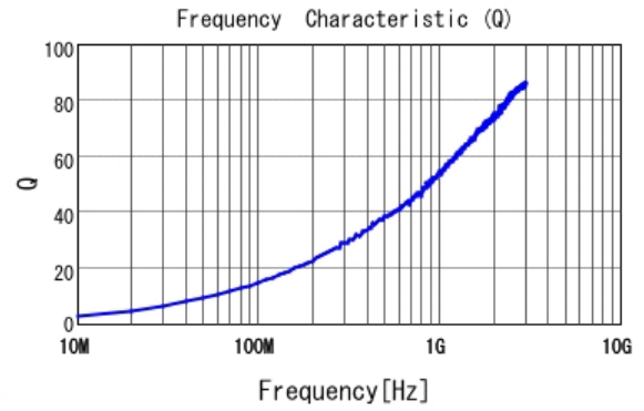
■ LQP03HQ1N8W02 Q
