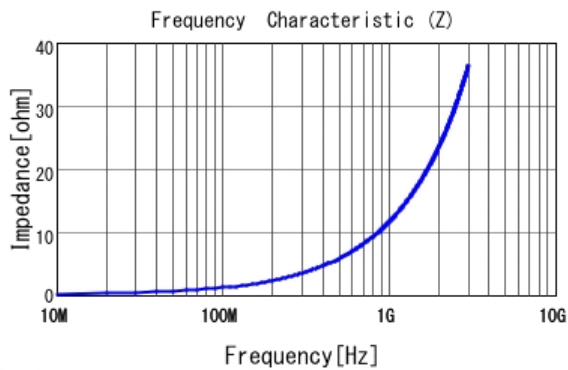
■ LQP03HQ1N8W02 |Z|
