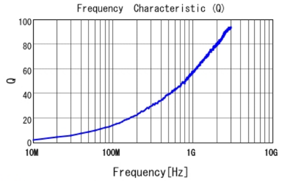
■ LQP03HQ1N7B02 Q
