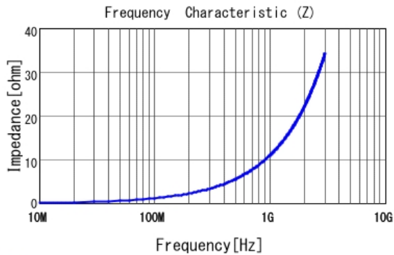
■ LQP03HQ1N7B02 |Z|
