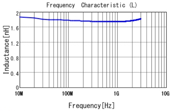
■ LQP03HQ1N7B02 L
