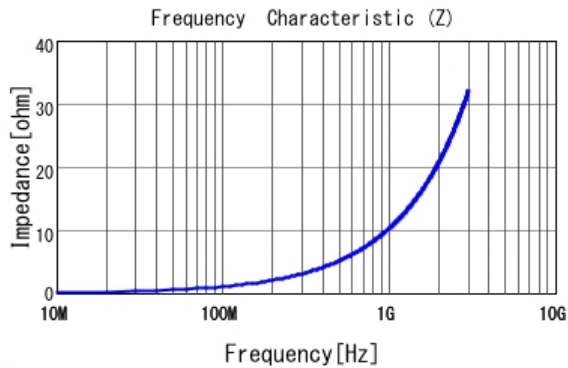
■ LQP03HQ1N6W02 |Z|
