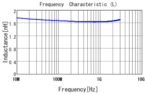
■ LQP03HQ1N6W02 L
