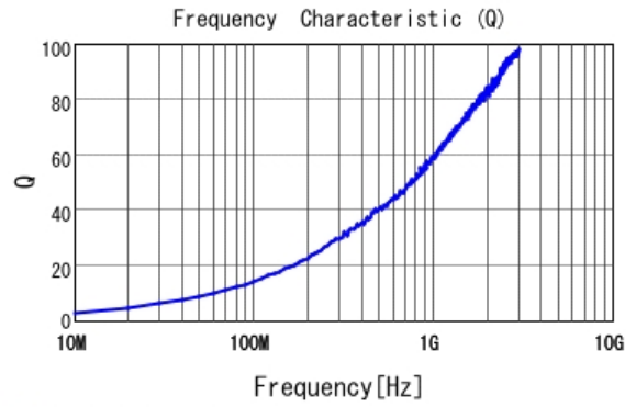
■ LQP03HQ1N6W02 Q
