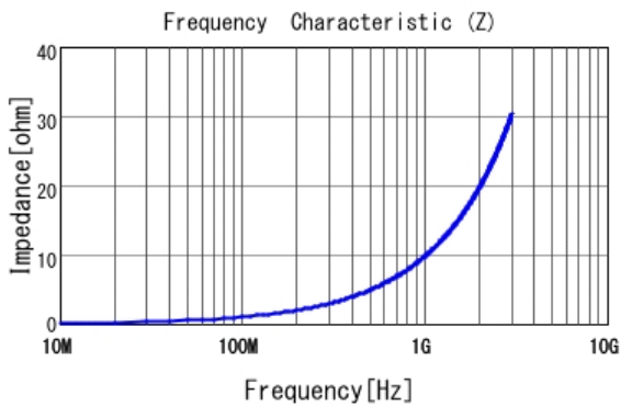
■ LQP03HQ1N5W02 |Z|
