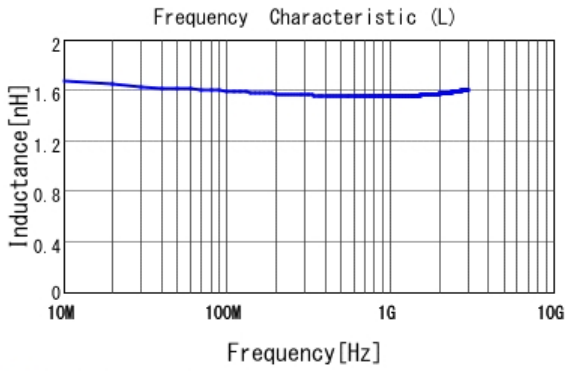
■ LQP03HQ1N5W02 L
