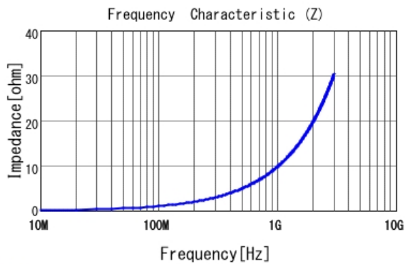
■ LQP03HQ1N5B02 |Z|
