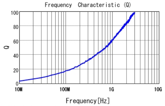
■ LQP03HQ1N5B02 Q
