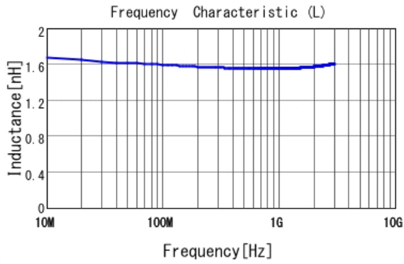
■ LQP03HQ1N5B02 L
