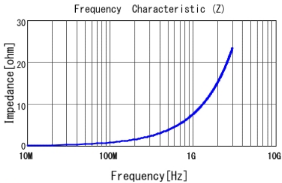
■ LQP03HQ1N2C02 |Z|
