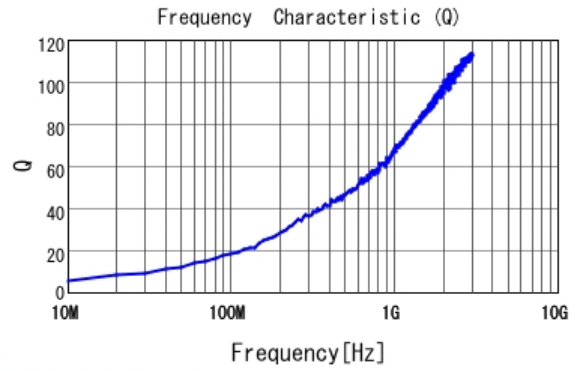
■ LQP03HQ1N2C02 Q
