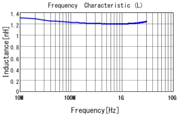
■ LQP03HQ1N2C02 L
