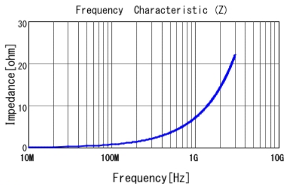
■ LQP03HQ1N1W02 |Z|
