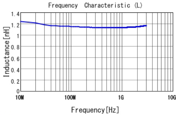
■ LQP03HQ1N1W02 L
