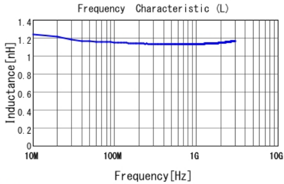
■ LQP03HQ1N1B02 L
