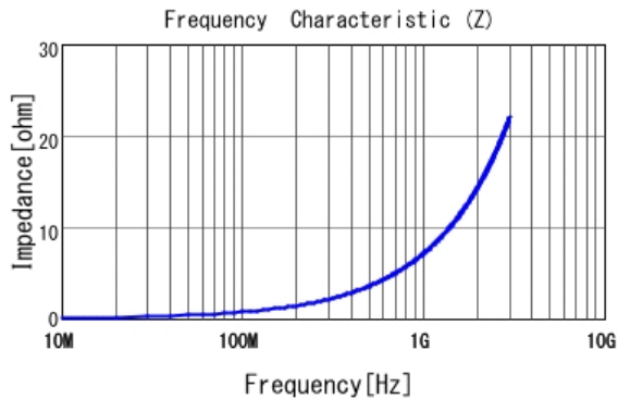
■ LQP03HQ1N1B02 |Z|
