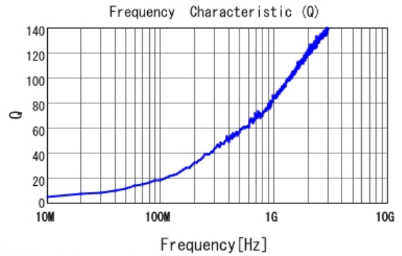
■ LQP03HQ1N1B02 Q
