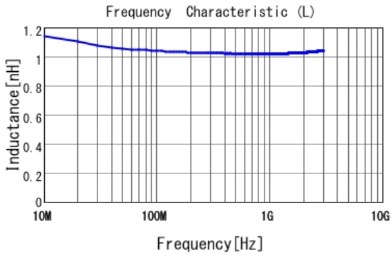
■ LQP03HQ1N0B02 L
