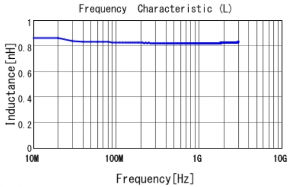
■ LQP03HQ0N8B02 L
