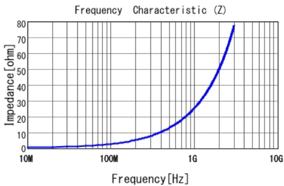
■ LQP02TQ4N1B02 |Z|
