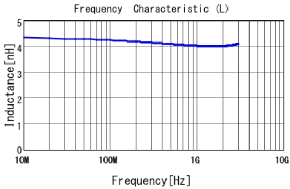
■ LQP02TQ4N1B02 L
