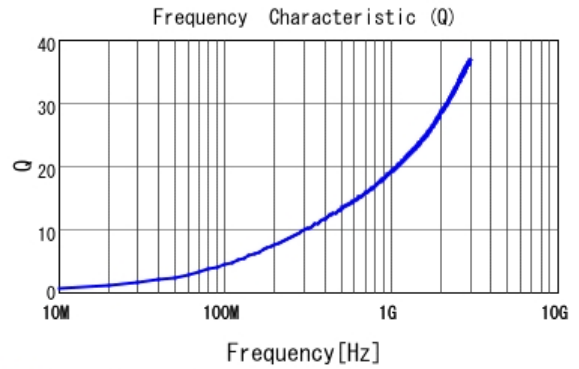
■ LQP02TQ4N1B02 Q
