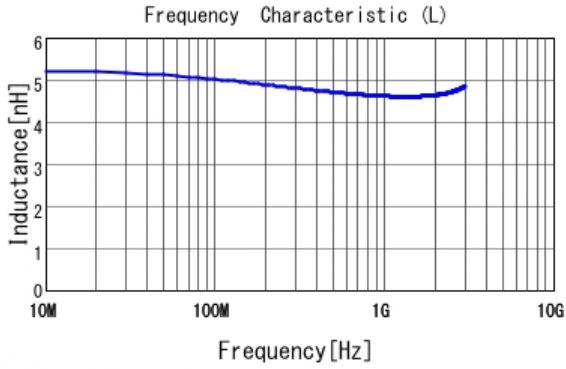
■ LQP02TN4N7H02 L
