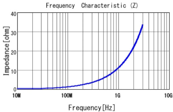
■ LQP02TN1N8B02 |Z|
