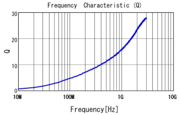
■ LQP02TN1N8B02 Q
