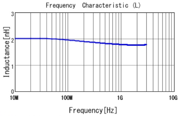
■ LQP02TN1N8B02 L
