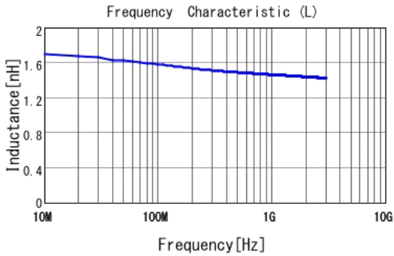
■ LQP02HQ1N5W02 L
