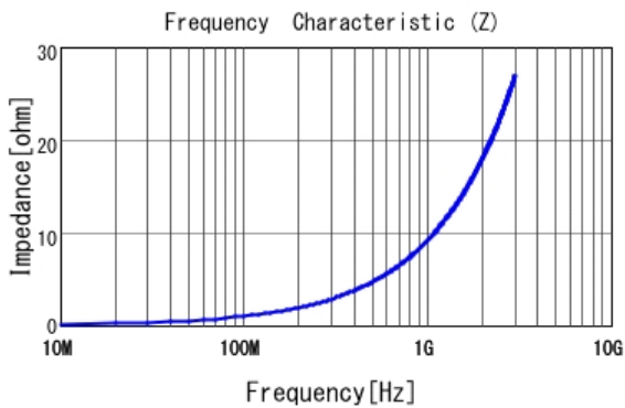
■ LQP02HQ1N5W02 |Z|
