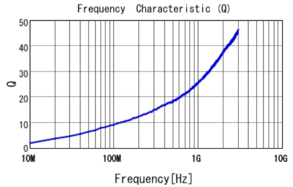
■ LQP02HQ1N5W02 Q
