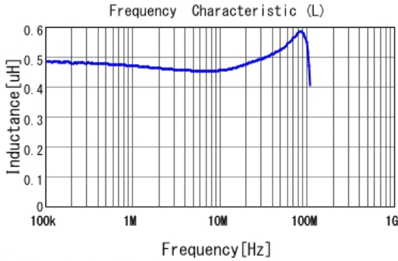
LQM31PNR47M00 L
