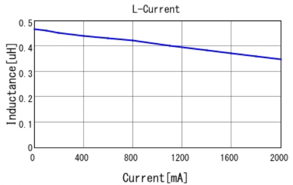
LQM31PNR47M00 L-Current 20degC
