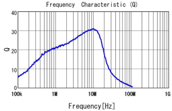
LQM31PNR47M00 Q
