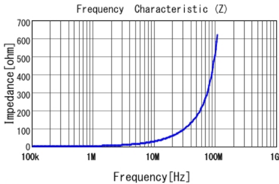
LQM31PNR47M00 |Z|
