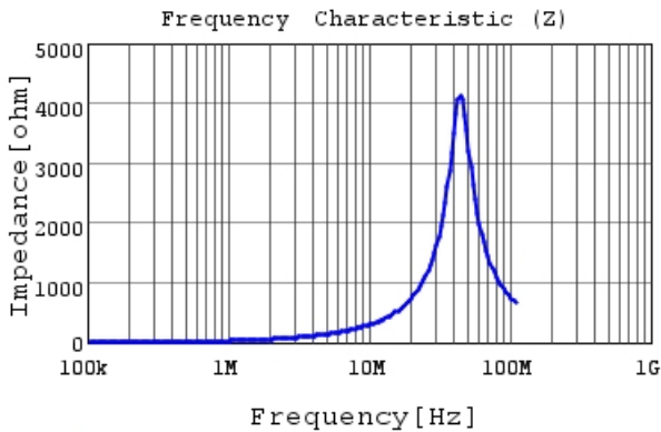
LQM31PN4R7M00 |Z|
