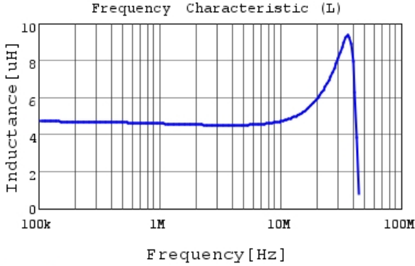
LQM31PN4R7M00 L
