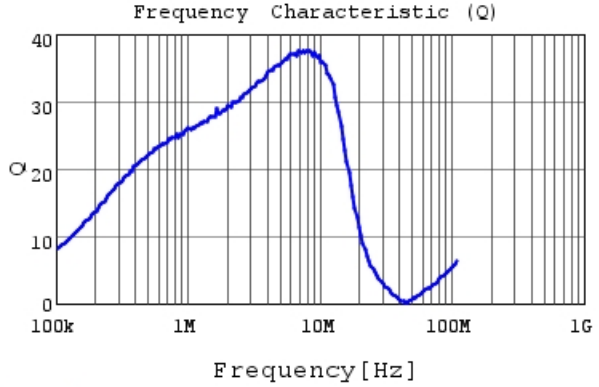
LQM31PN4R7M00 Q
