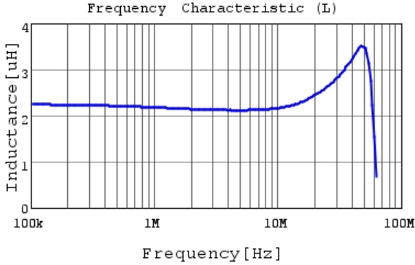
LQM31PN2R2M00 L
