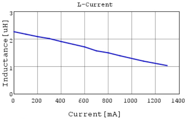
LQM31PN2R2M00 L-Current 20degC
