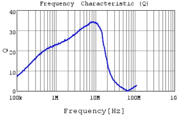
LQM31PN2R2M00 Q
