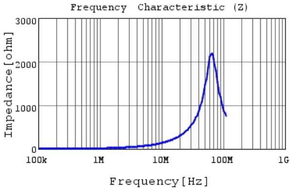
LQM31PN2R2M00 |Z|
