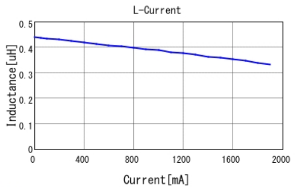
■ LQM2MPZR47NG0 L-Current 20degC
