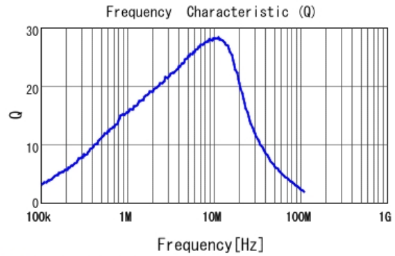
■ LQM2MPZR47NG0 Q
