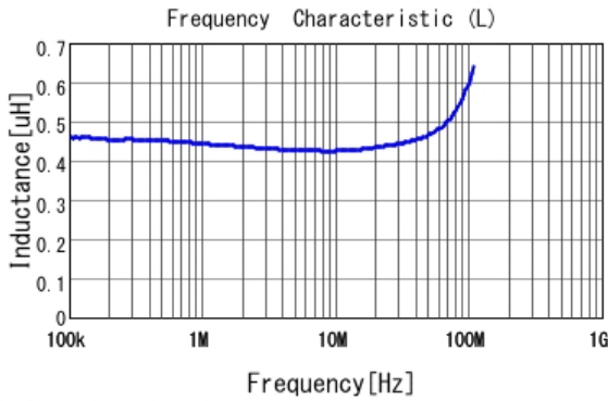
■ LQM2MPZR47NG0 L
